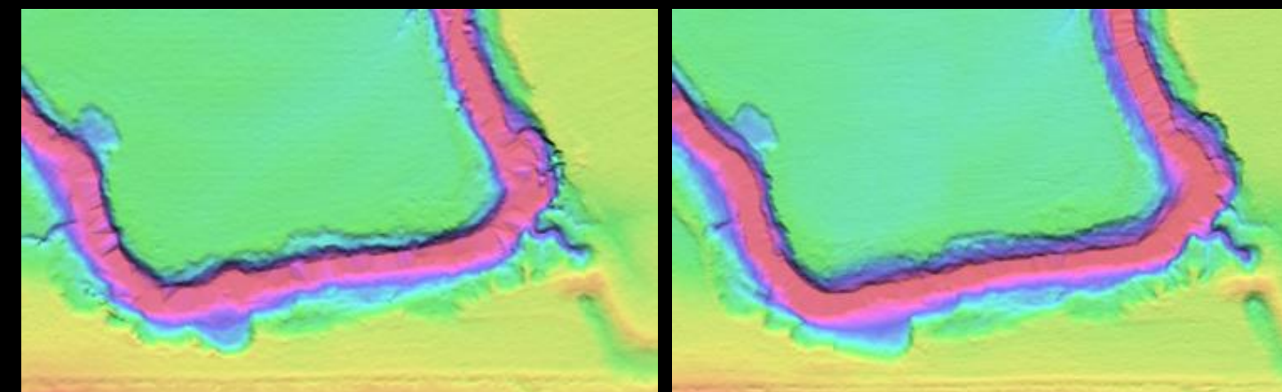
Figure 3: LiDAR DEM from 2009 (left) and 2017 (right) – CATALYST algorithms were used to examine the changes in elevation (Figure 2).
